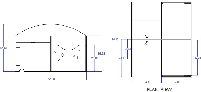
Double-Faced Family Workstation
